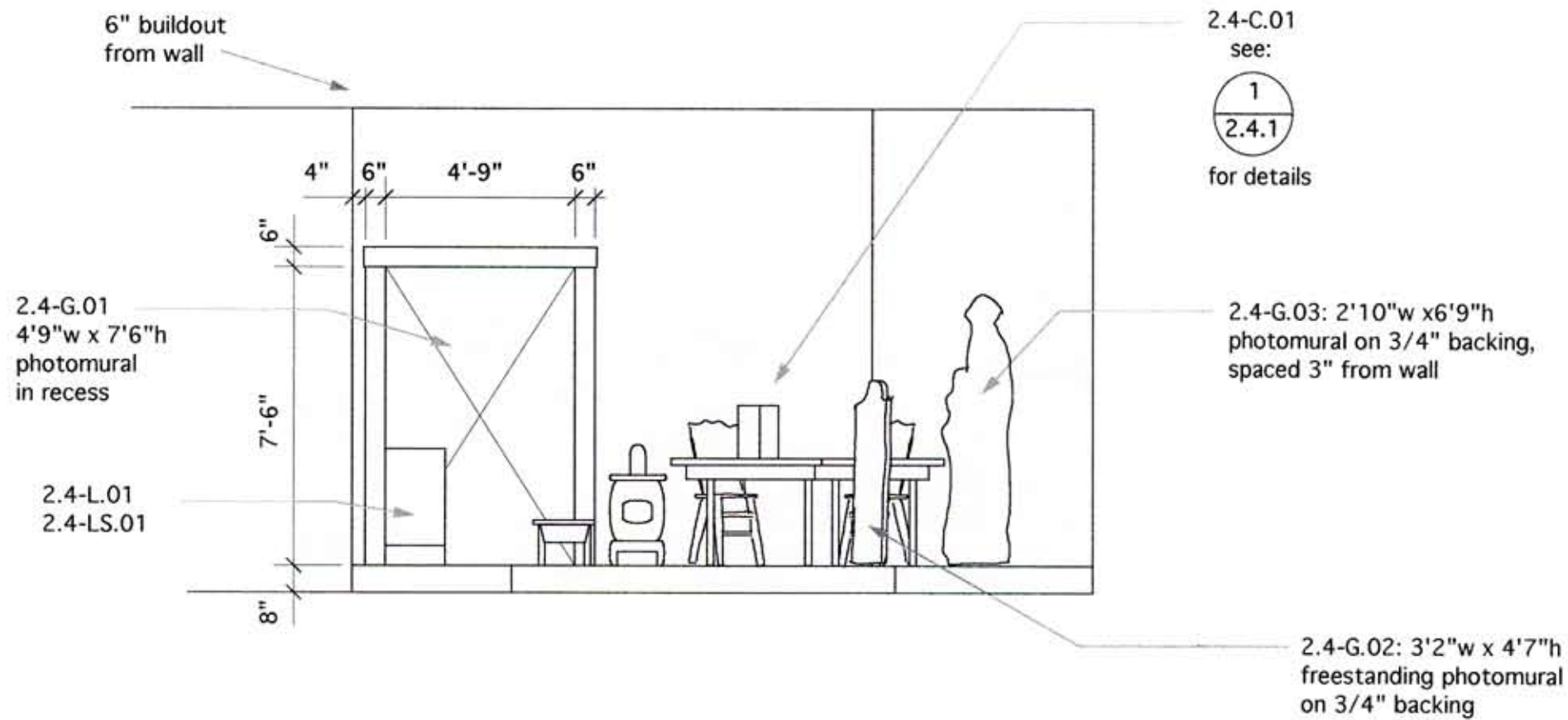
1 elevation, kitchen platform 2.4 scale: 1/4" = 1'-0"
